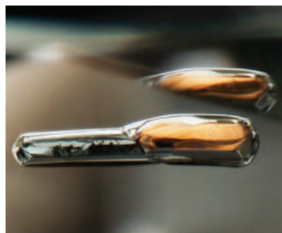
Figure 8. Contact inclusions of grayish blue omphacite and orange pyrope-almandine garnet confirmed the eclogitic origin of this 2.03 ct Fancy yellow-green diamond. Also observed was graphite along the interface between the inclusions and diamond host. Image width: 1.22 mm.
