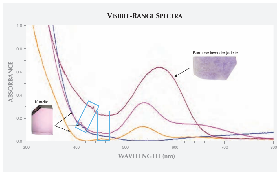
Figure 5. As these UV-visible absorption spectra demonstrate, polycrystalline Burmese lavender jadeite and single-crystalline pink spodumene (kunzite) share similar weak narrow bands (blue boxes) between 400 and 460 nm and similar broad bands above 500. The single-crystal kunzite spectra were collected from the three orthogonal orientations that displayed the most pleochroism, ranging from pink (pink line) to light pink (orange line) and very light blue-green (blue line).
