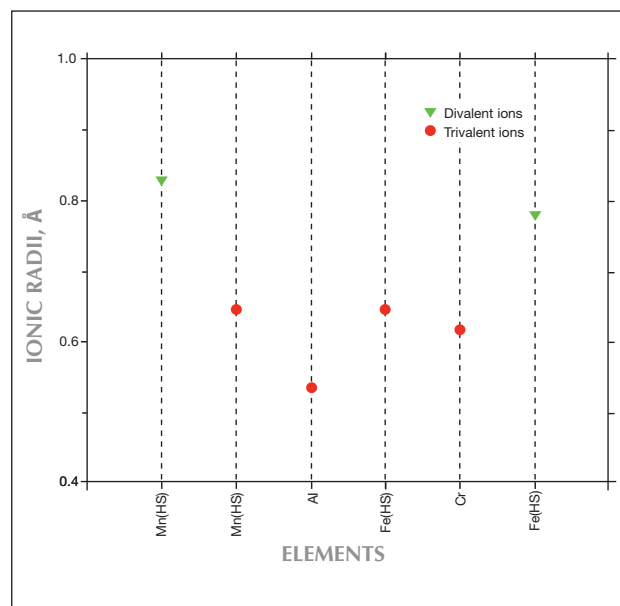
Figure 6. Ionic radii of trivalent ions such as Mn, Fe, and Cr (isovalent to \text{Al}^{3+} , in solid circles) closely match those of \text{Al}^{3+} and can readily replace \text{Al}^{3+} as chromophore ions. Divalent ions (aliovalent to \text{Al}^{3+} , in solid triangles) are less suited in terms of size and charge balance. The label “HS” represents high-spin configuration. Data for ionic radii of six coordinated ions are based on Shannon (1976).
