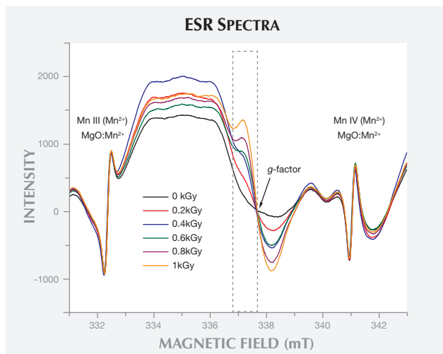
Figure 5. These ESR spectra show a South Sea cultured pearl's nacre (left) and nucleus (right) before and after irradiation up to 1 kGy. These spectra were obtained for a single cultured pearl irradiated with different doses. \text{CO}_2^- radicals appeared as irradiation doses increased in both the nacre (left) and nucleus (right). Nucleus spectra (right) show a large unassigned signal in the 333–337 mT range, both before and after irradiation.
