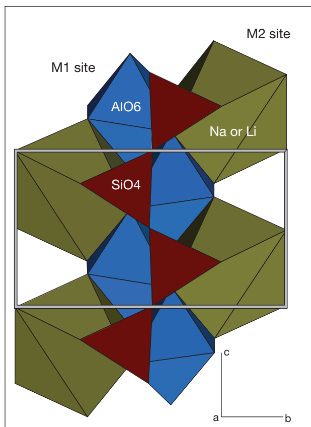
Figure 3. This view of the crystal structure of jadeite and spodumene illustrates the basic building blocks: \text{AlO}_6 octahedra and \text{SiO}_4 tetrahedra, and their geo- metric relationships (based on structural refinement data of Cameron et al., 1973). The crystallographic orientation is shown in the lower right corner pro- jected down the a -axis.
